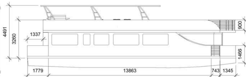
STARBOARD ELEVATION SCALE 1:100
