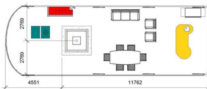
UPPER DECK PLAN 4 CABIN HOUSE BOAT SCALE 1:100
