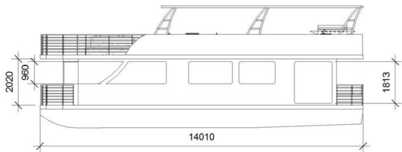
PORT SIDE ELEVATION 2 1/2 CABIN HOUSE BOAT 1:100
