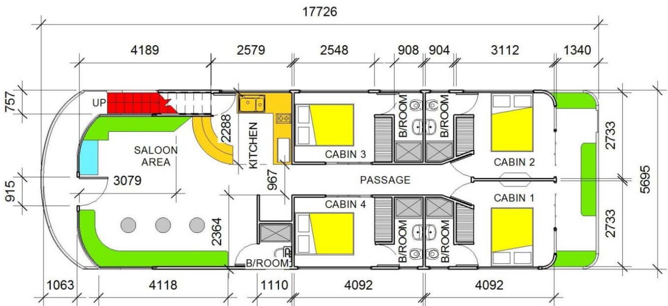
FLOOR PLAN 4 CABIN HOUSE BOAT
